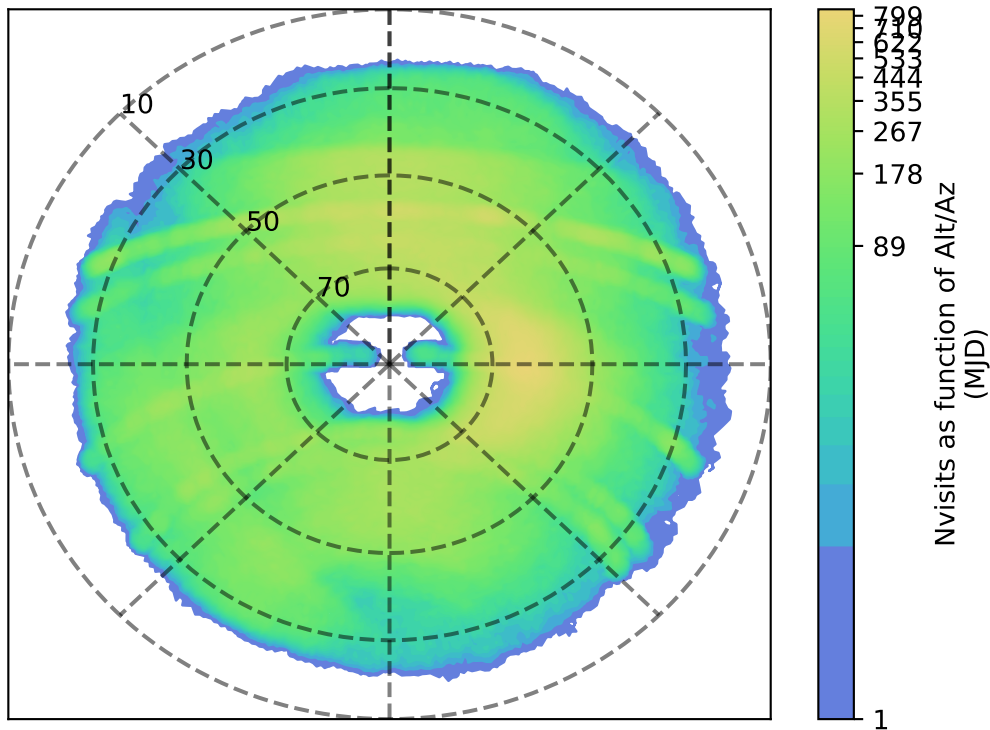
ddf_loaded_half_fl15_v3.4_10yrs g: Nvisits as function of Alt/Az
