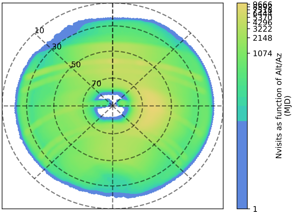
ddf_loaded_half_fl15_v3.4_10yrs : Nvisits as function of Alt/Az
