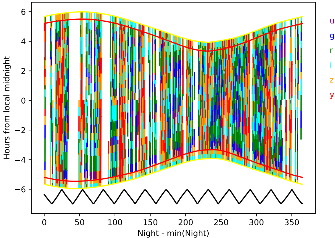
ddf_loaded_half_fl15_v3.4_10yrs year 4-5: Hourglass
