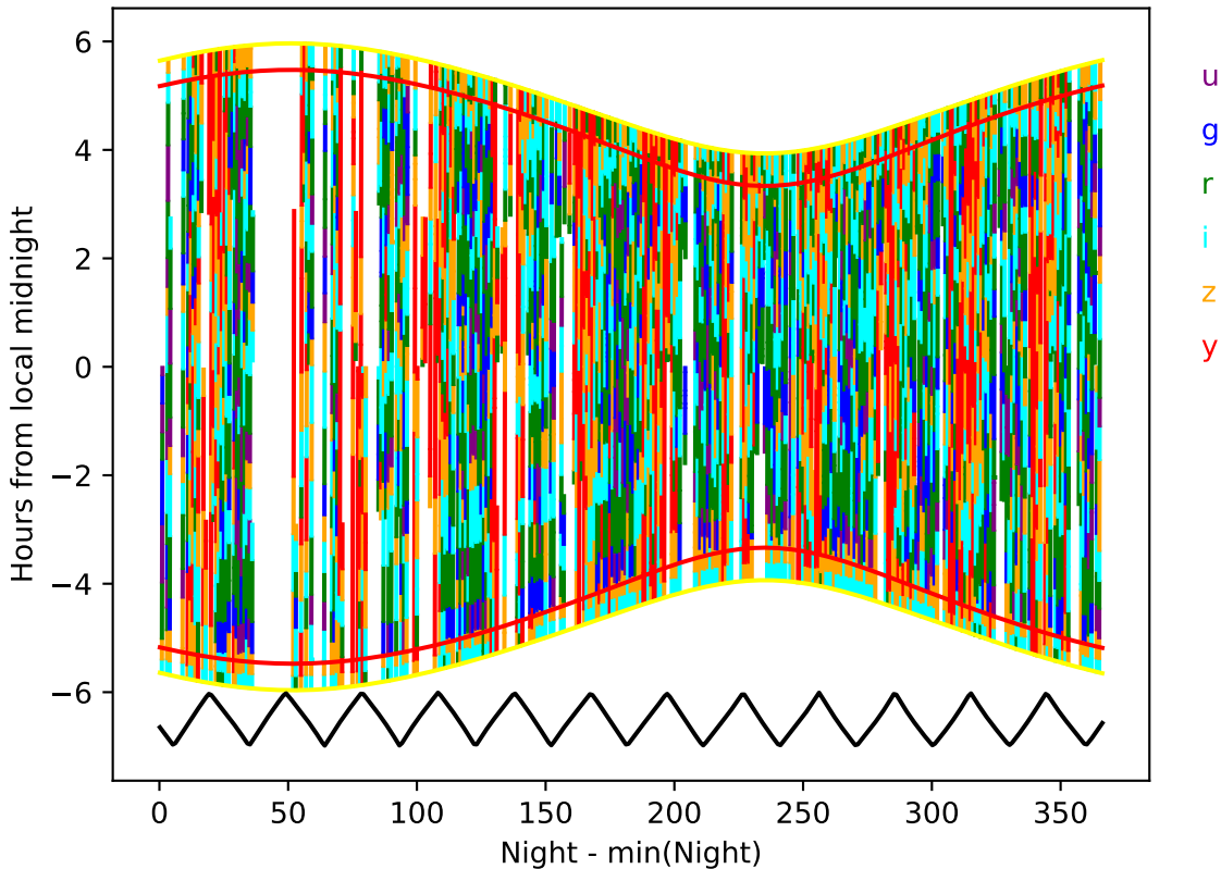
ddf_loaded_half_fl15_v3.4_10yrs year 2-3: Hourglass
