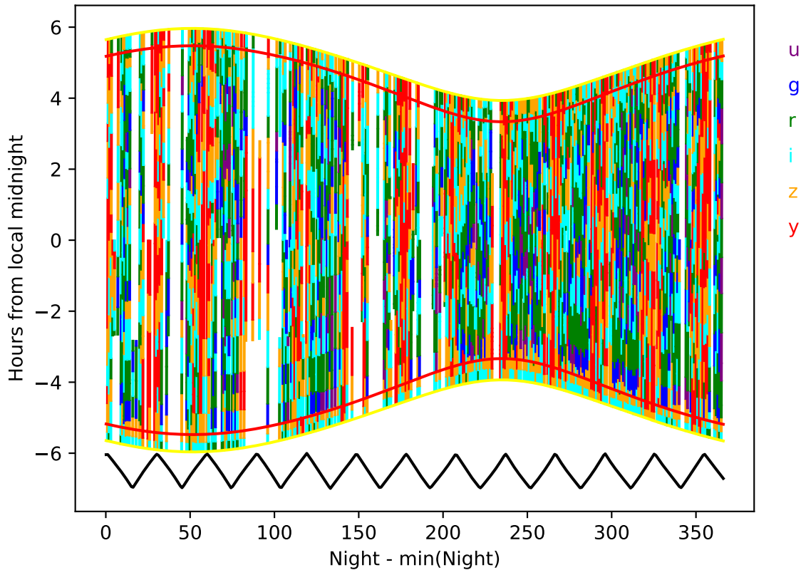
ddf_loaded_half_fl15_v3.4_10yrs year 1-2: Hourglass
