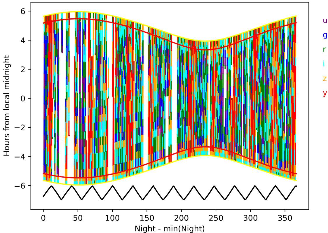
ddf_loaded_half_fl15_v3.4_10yrs year 0-1: Hourglass
