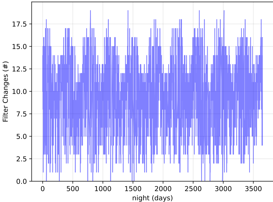
ddf_loaded_half_fl15_v3.4_10yrs : Filter Changes
