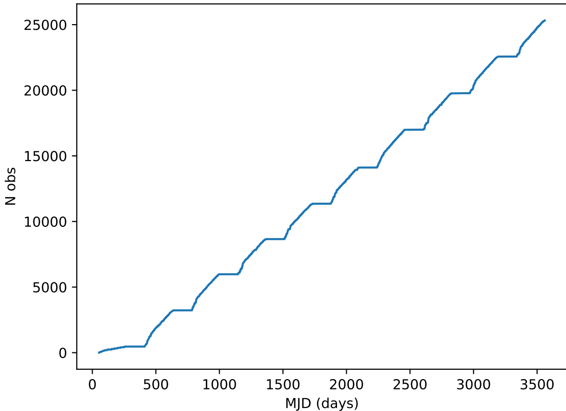
ddf_loaded_half_fl15_v3.4_10yrs note like DD:ELAISS1%: Cumulative
