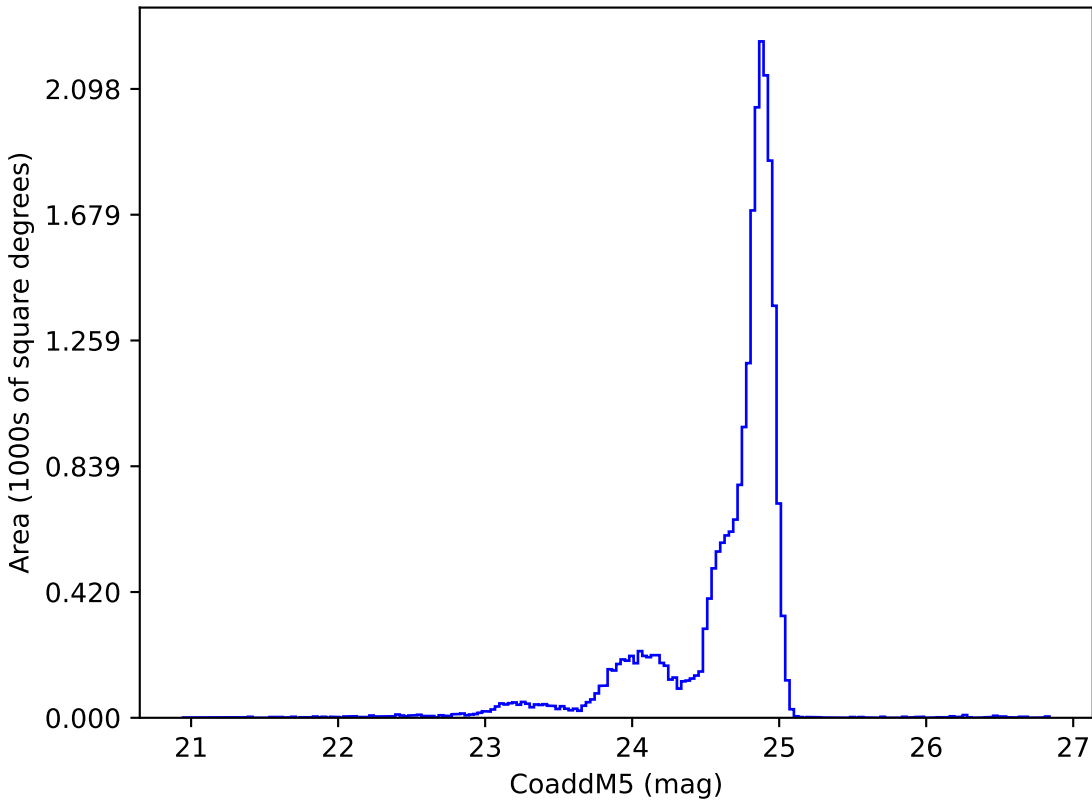
ddf_loaded_half_fl15_v3.4_10yrs y: CoaddM5
