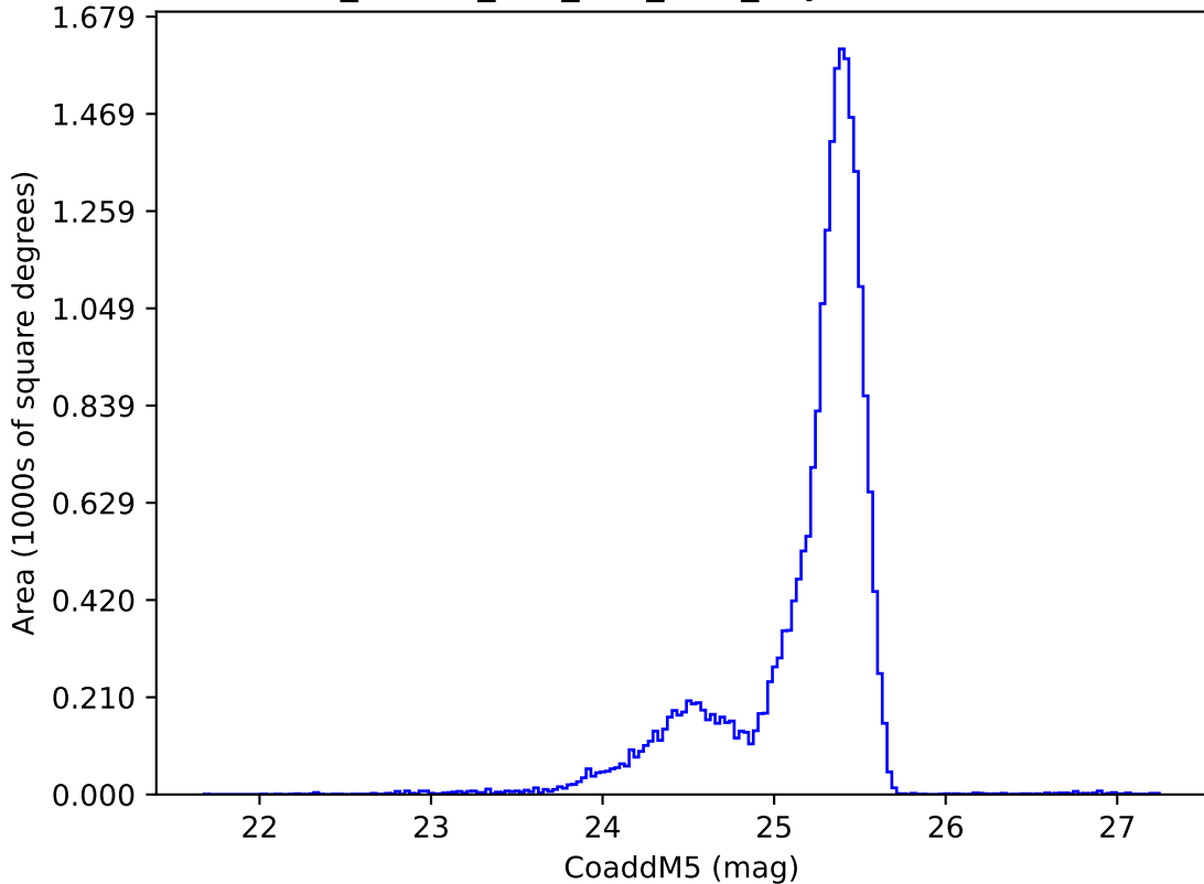
ddf_loaded_half_fl15_v3.4_10yrs u: CoaddM5
