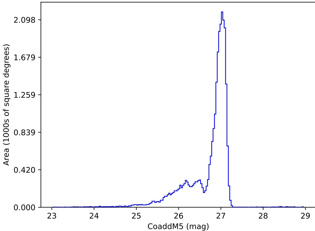
ddf_loaded_half_fl15_v3.4_10yrs r: CoaddM5
