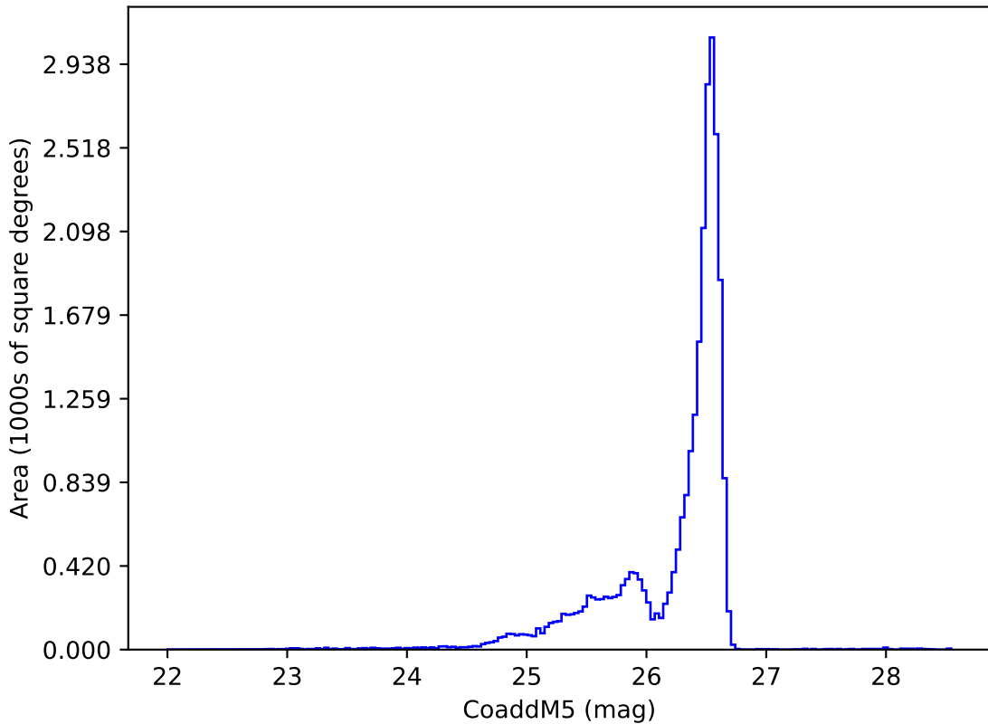
ddf_loaded_half_fl15_v3.4_10yrs i: CoaddM5
