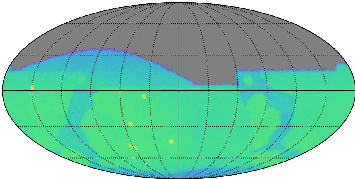
ddf_loaded_half_fl15_v3.4_10yrs g: CoaddM5
