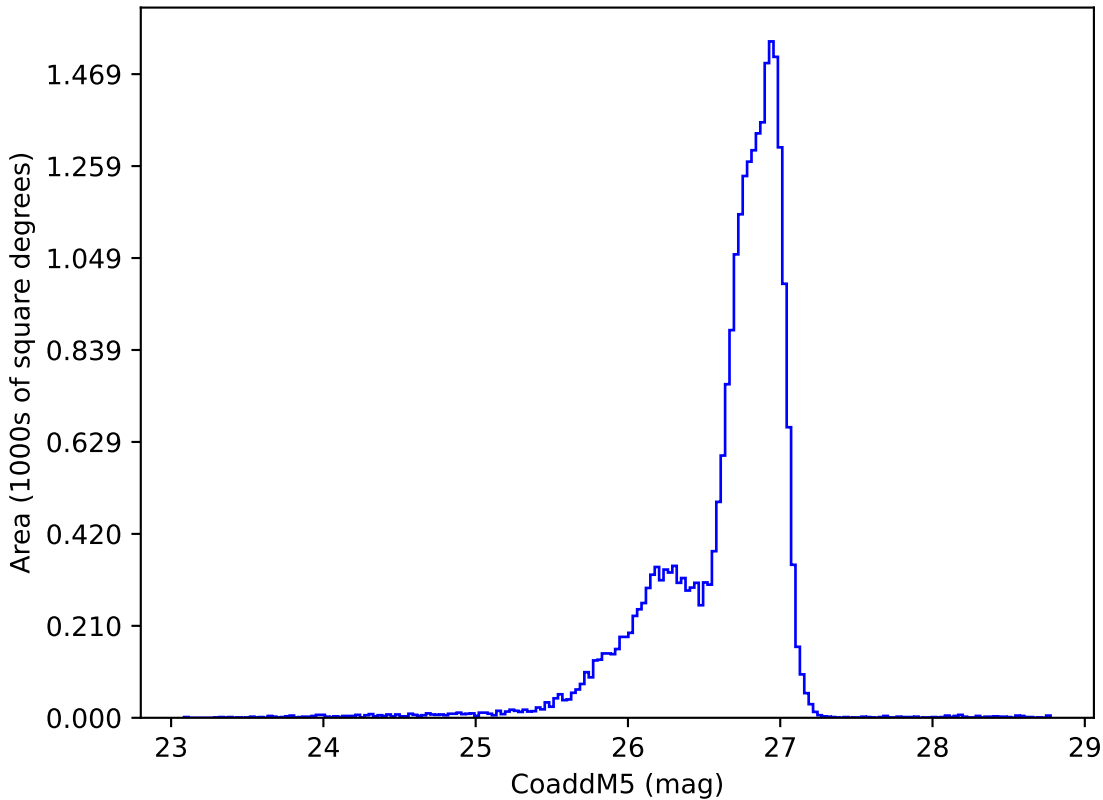
ddf_loaded_half_fl15_v3.4_10yrs g: CoaddM5
