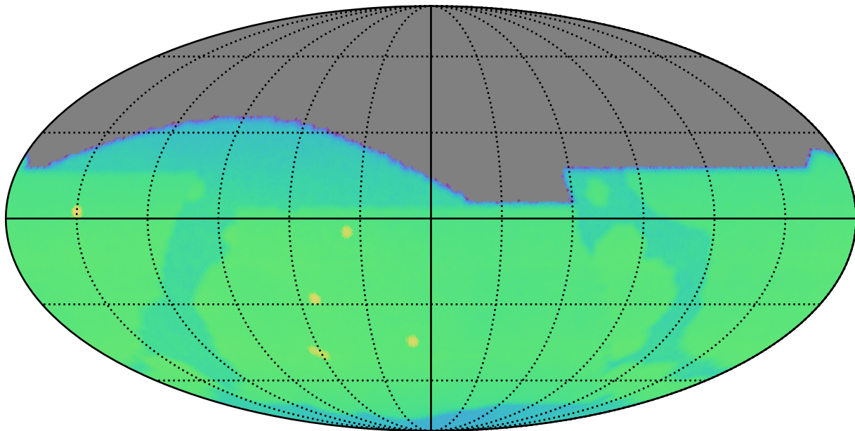
ddf_loaded_half_f15_v3.4_10yrs : CoaddM5
