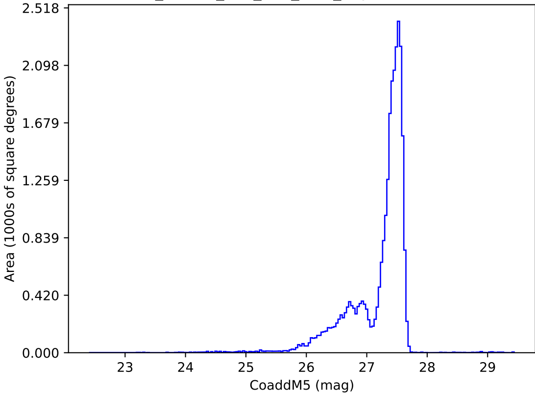
ddf_loaded_half_fl15_v3.4_10yrs : CoaddM5
