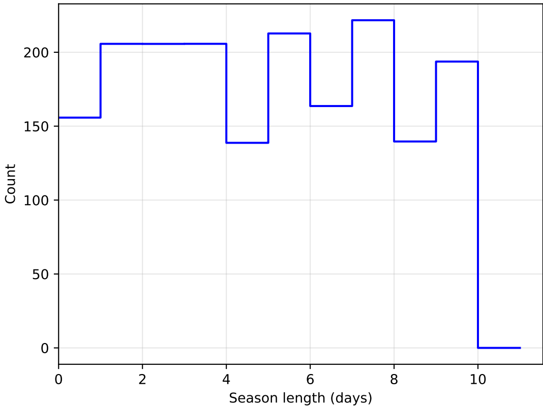
ddf_loaded_half_fl15_v3.4_10yrs DD:WFD all bands: SeasonLength
