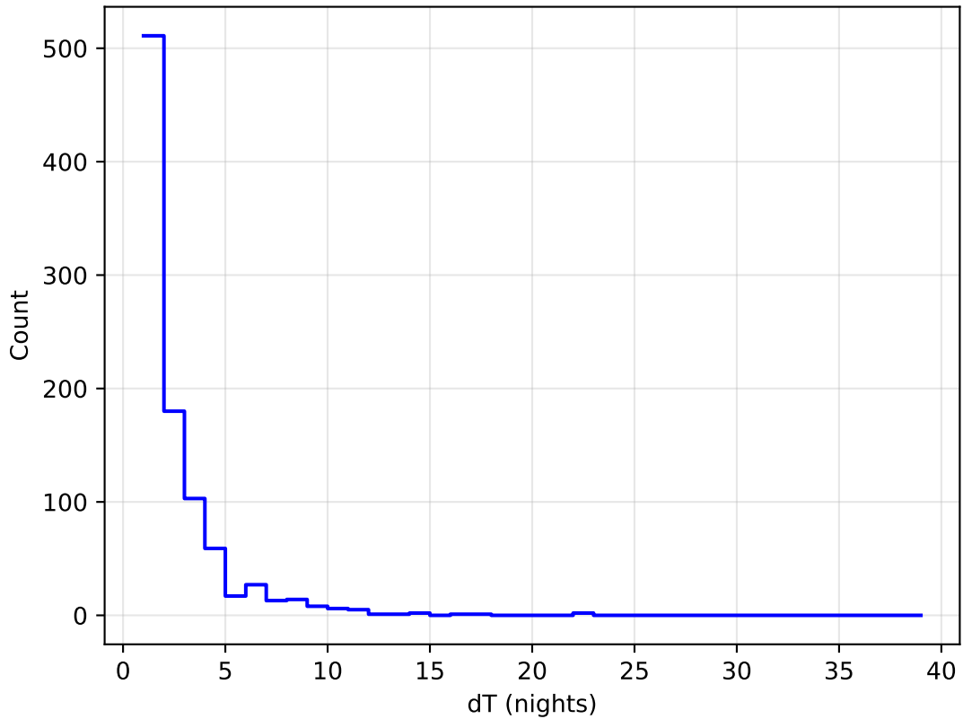
ddf_loaded_half_fl15_v3.4_10yrs all bands: DD:XMM_LSS Delta Nights Histogram
