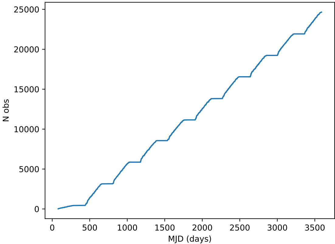
ddf_loaded_half_fl15_v3.4_10yrs all bands: DD:XMM_LSS Cumulative NVisits
