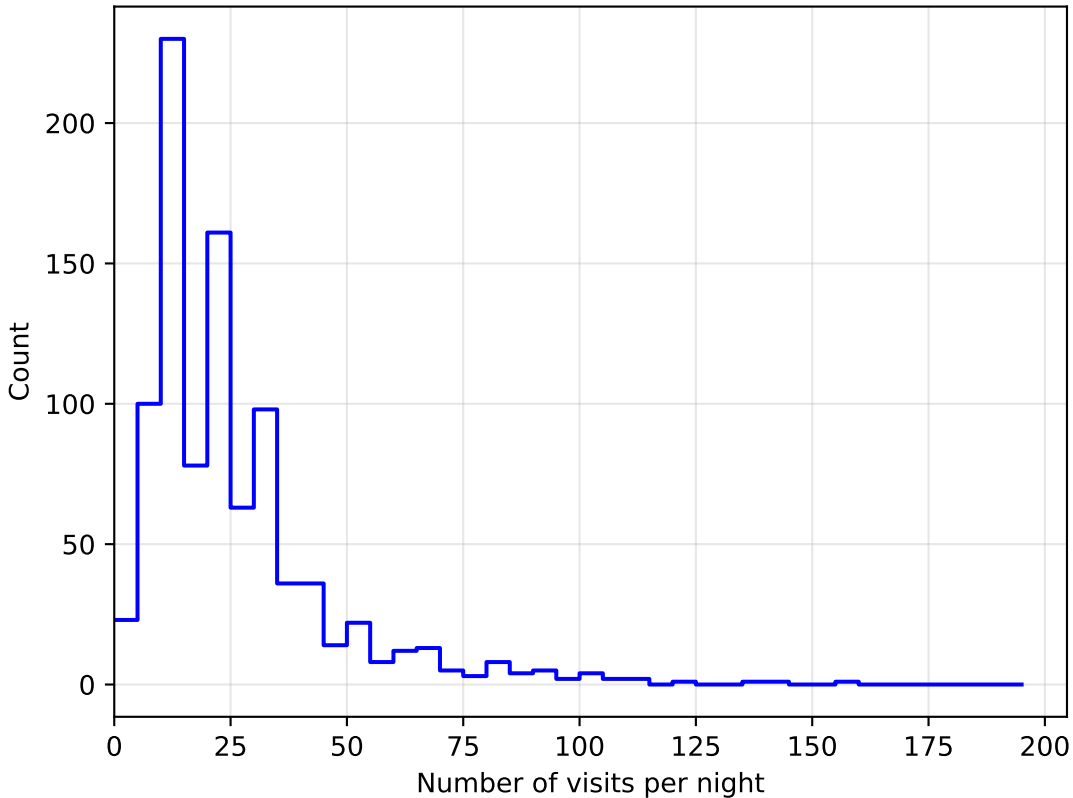
ddf_loaded_half_fl15_v3.4_10yrs all bands: DD:ELAISS1 NVisitsPerNight
