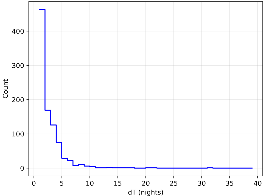
ddf_loaded_half_fl15_v3.4_10yrs all bands: DD:ELAISS1 Delta Nights Histogram
