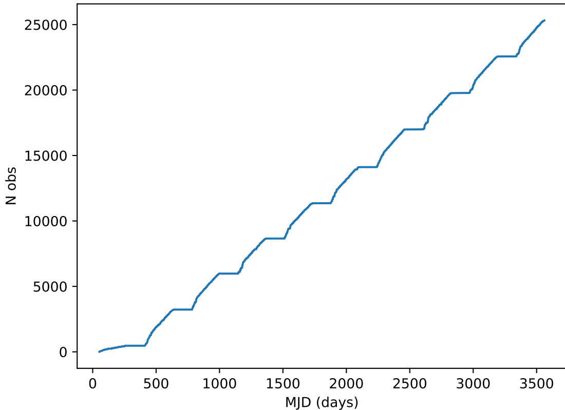
ddf_loaded_half_fl15_v3.4_10yrs all bands: DD:ELAISS1 Cumulative NVisits
