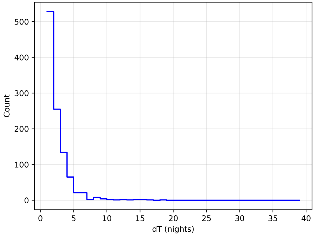
ddf_loaded_half_fl15_v3.4_10yrs all bands: DD:EDFS Delta Nights Histogram
