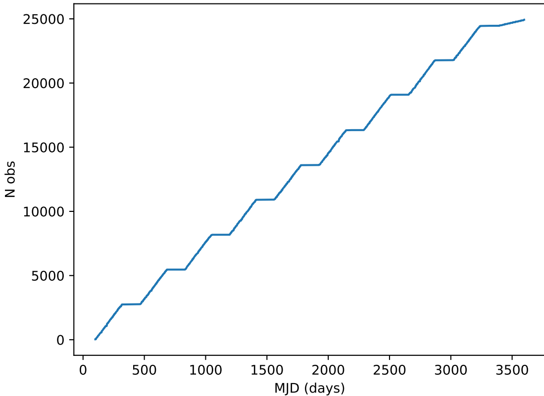
ddf_loaded_half_fl15_v3.4_10yrs all bands: DD:EDFS Cumulative NVisits
