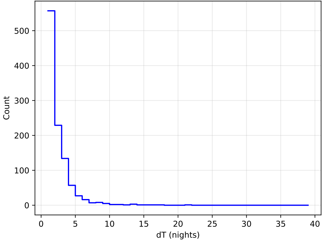
ddf_loaded_half_fl15_v3.4_10yrs all bands: DD:ECDFS Delta Nights Histogram
