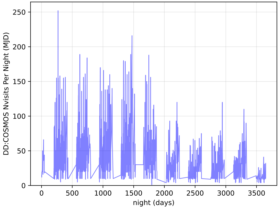
ddf_loaded_half_fl15_v3.4_10yrs all bands: DD:COSMOS Nvisits Per Night
