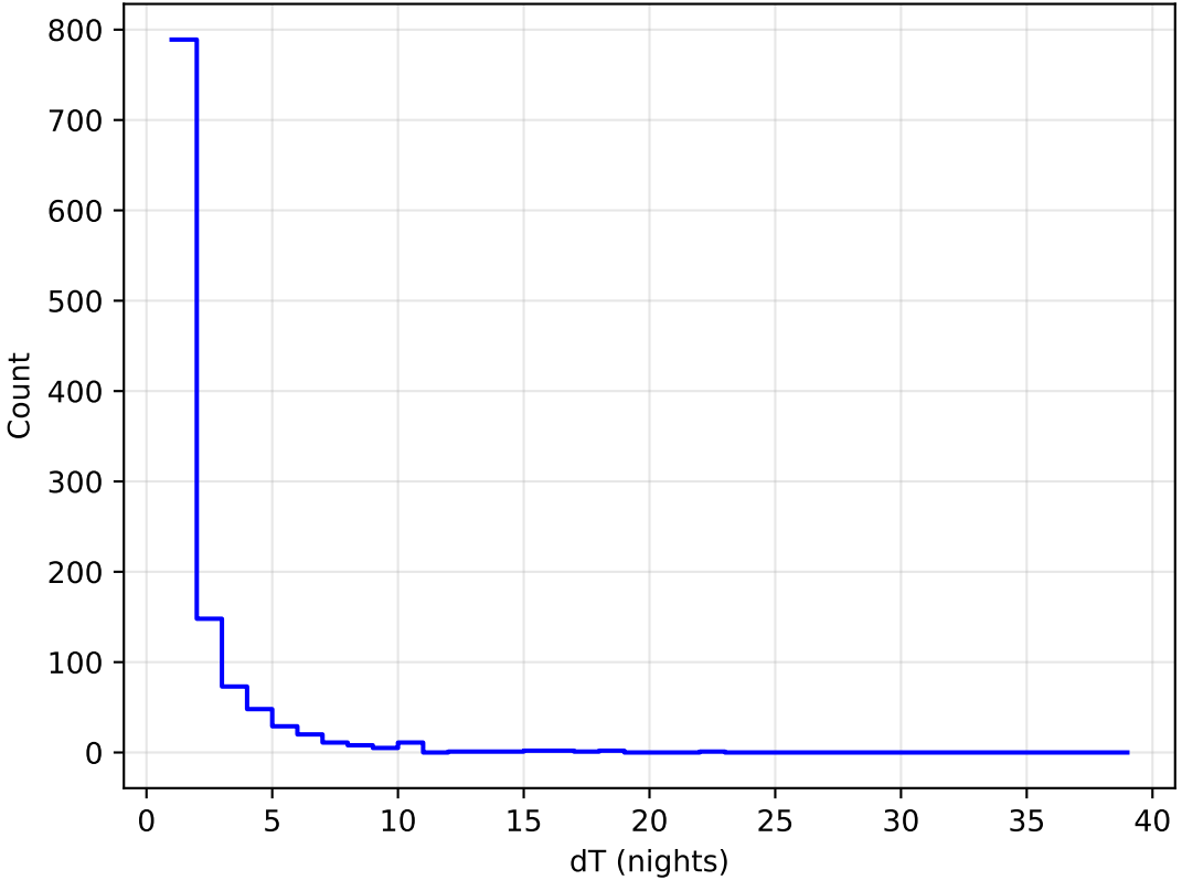
ddf_loaded_half_fl15_v3.4_10yrs all bands: DD:COSMOS Delta Nights Histogram
