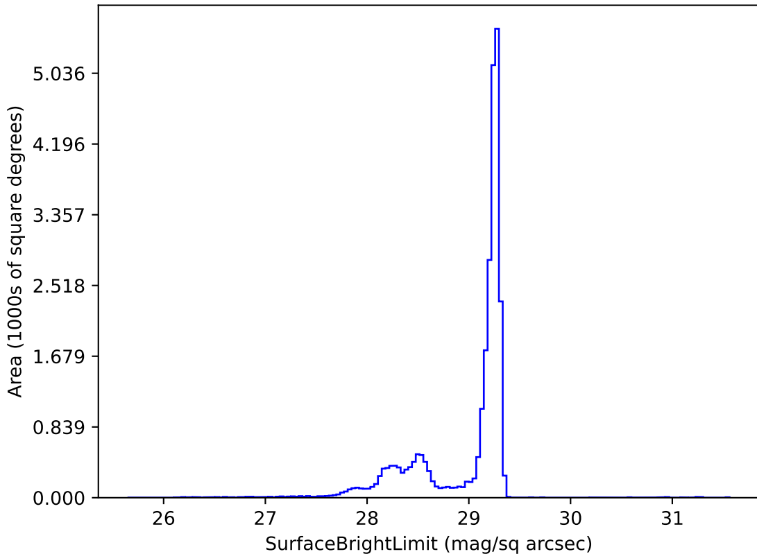
ddf_loaded_half_fl15_v3.3_10yrs z: SurfaceBrightLimit
