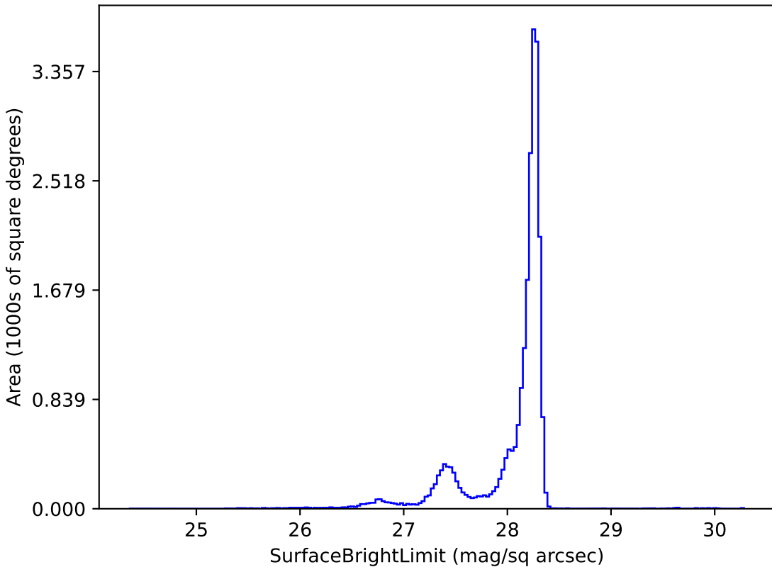
ddf_loaded_half_fl15_v3.3_10yrs y: SurfaceBrightLimit
