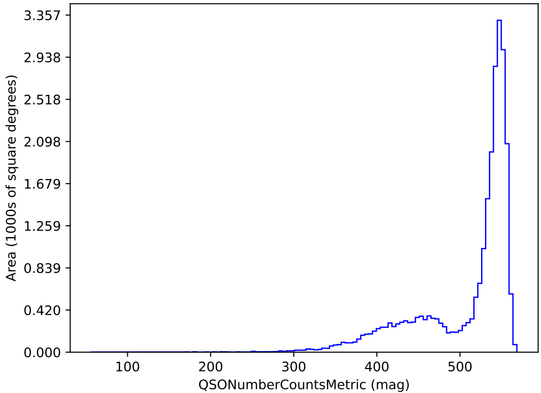
ddf_loaded_half_fl15_v3.3_10yrs i band and non-DD: QSONumberCountsMetric
