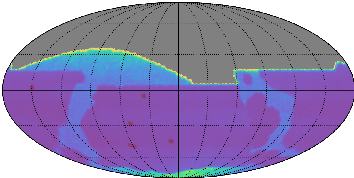
ddf_loaded_half_fl15_v3.3_10yrs : Proper Motion Uncert @ 20.5
