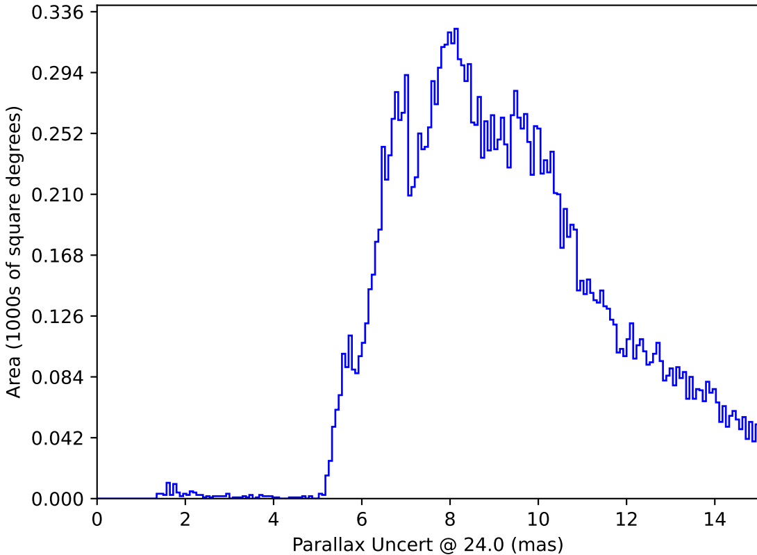
ddf_loaded_half_fl15_v3.3_10yrs : Parallax Uncert @ 24.0
