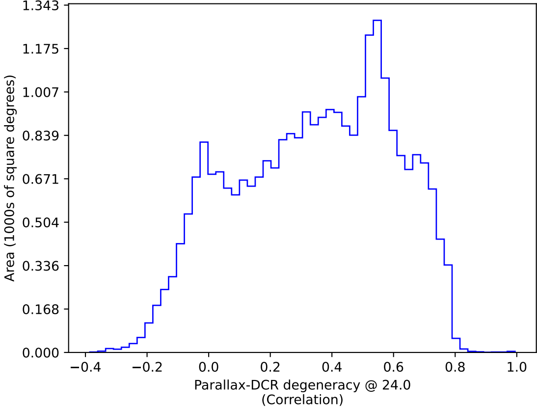
ddf_loaded_half_fl15_v3.3_10yrs : Parallax-DCR degeneracy @ 24.0
