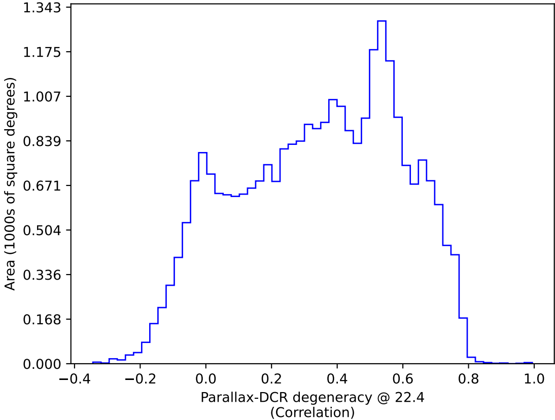
ddf_loaded_half_fl15_v3.3_10yrs : Parallax-DCR degeneracy @ 22.4
