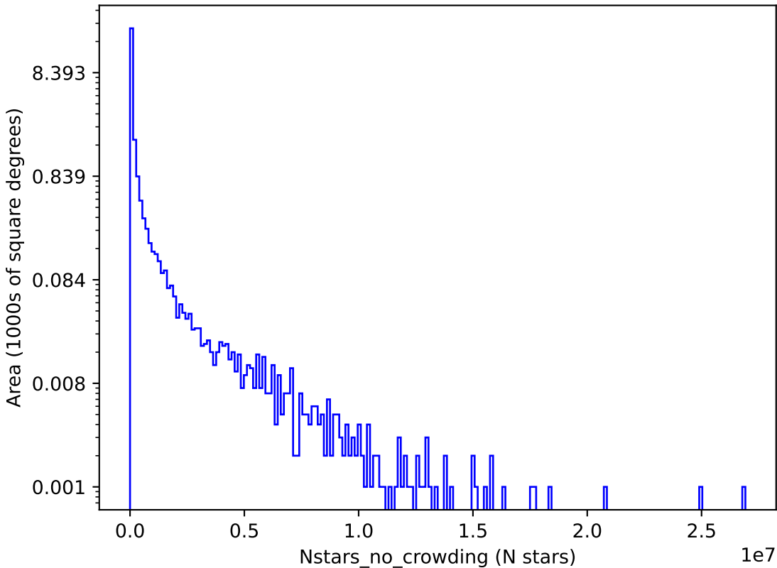
ddf_loaded_half_fl15_v3.3_10yrs z: Nstars_no_crowding
