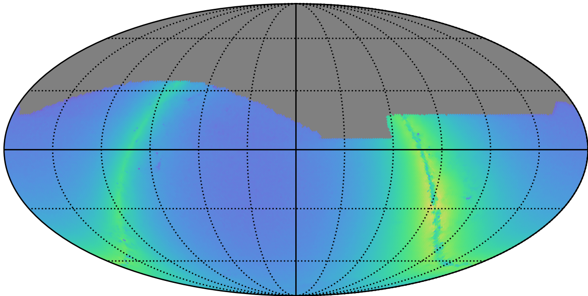
ddf_loaded_half_fl15_v3.3_10yrs i: Nstars_no_crowding
