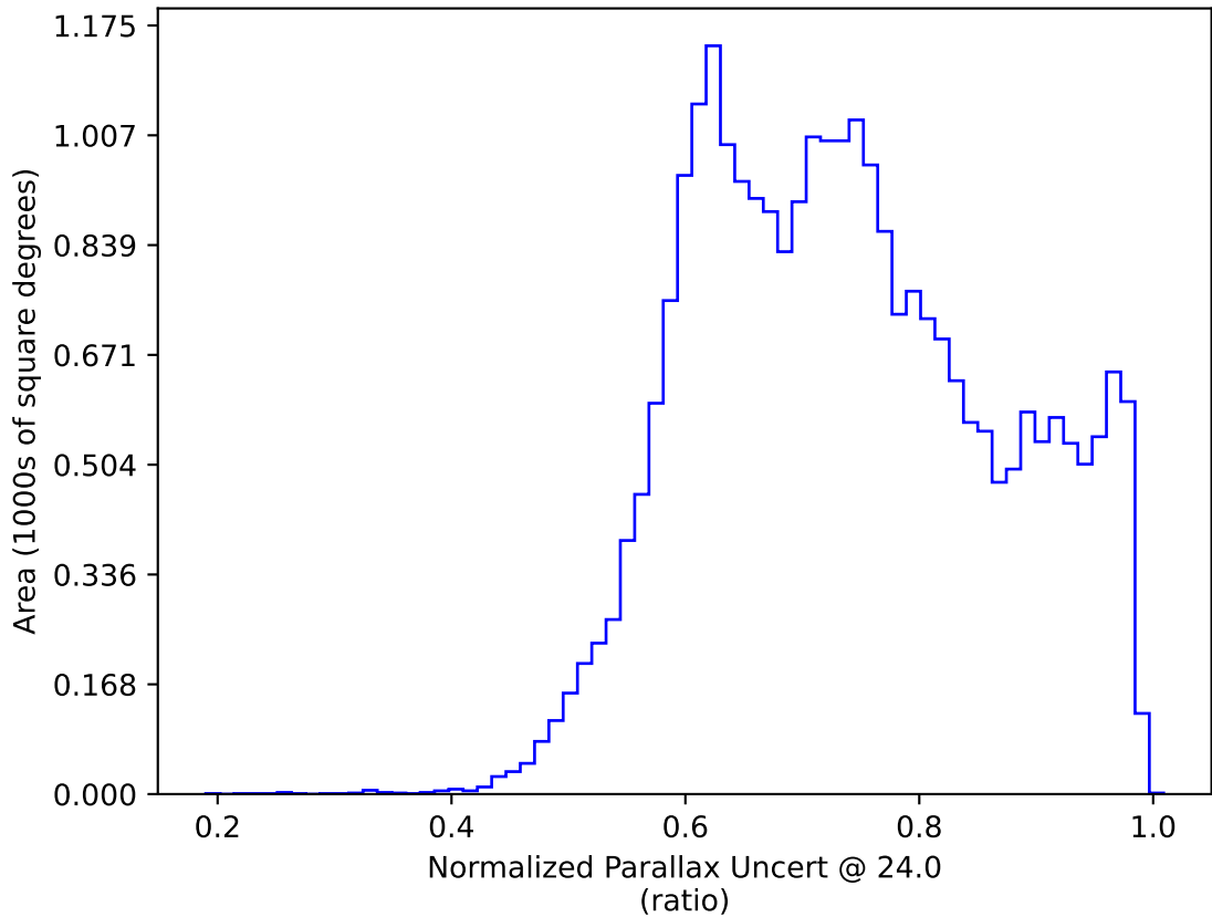
ddf_loaded_half_fl15_v3.3_10yrs : Normalized Parallax Uncert @ 24.0
