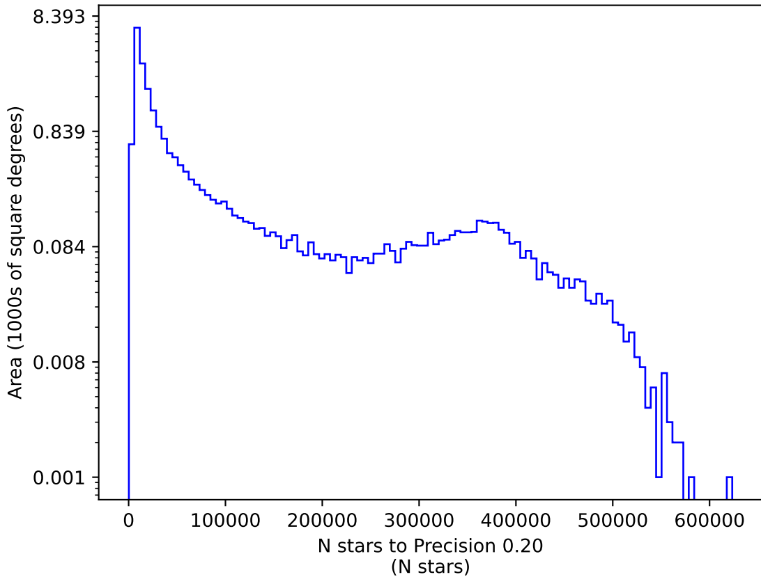
ddf_loaded_half_fl15_v3.3_10yrs y: N stars to Precision 0.20
