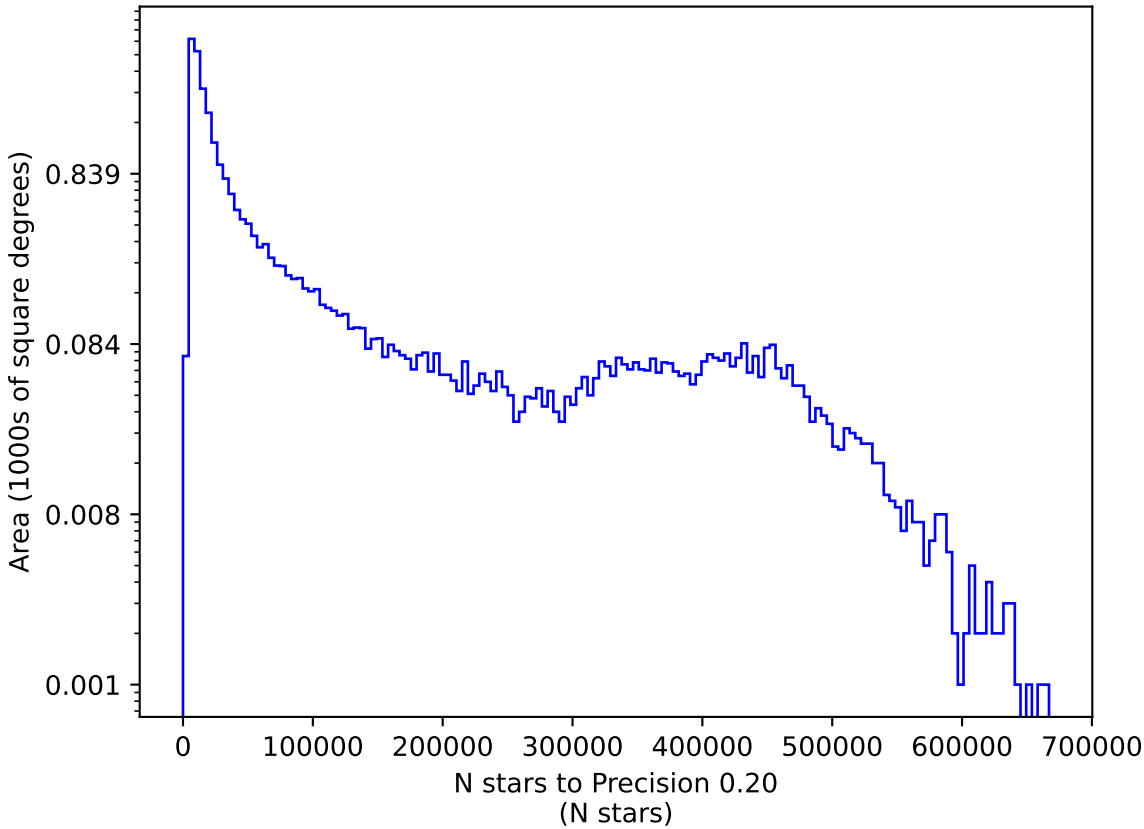
ddf_loaded_half_fl15_v3.3_10yrs r: N stars to Precision 0.20
