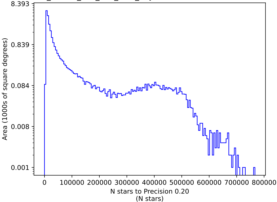
ddf_loaded_half_fl15_v3.3_10yrs i: N stars to Precision 0.20
