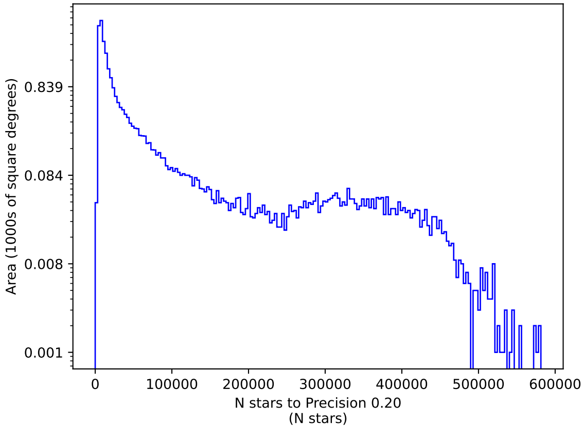
ddf_loaded_half_fl15_v3.3_10yrs g: N stars to Precision 0.20
