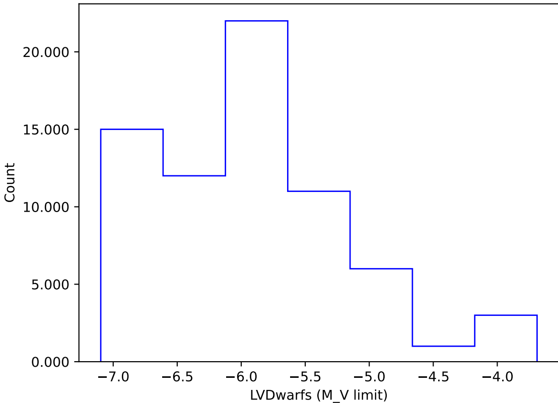
ddf_loaded_half_fl15_v3.3_10yrs gi: LVDwarfs
