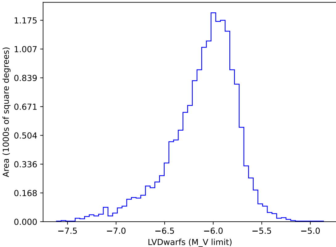
ddf_loaded_half_fl15_v3.3_10yrs gi: LVDwarfs
