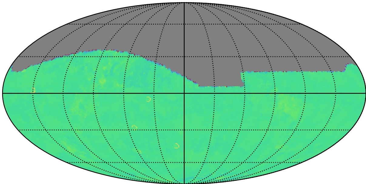
ddf_loaded_half_fl15_v3.3_10yrs z: Kuiper rotTelPos
