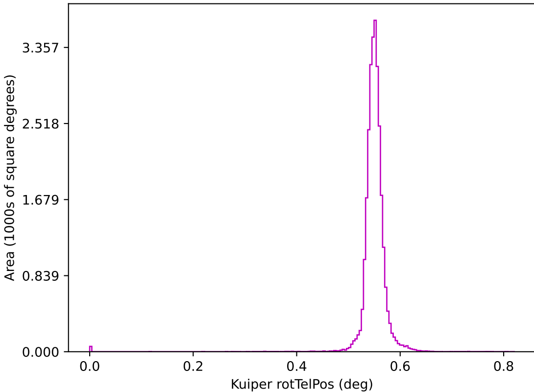
ddf_loaded_half_fl15_v3.3_10yrs z: Kuiper rotTelPos
