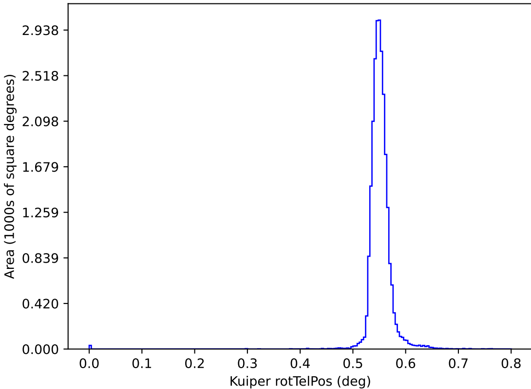
ddf_loaded_half_fl15_v3.3_10yrs y: Kuiper rotTelPos
