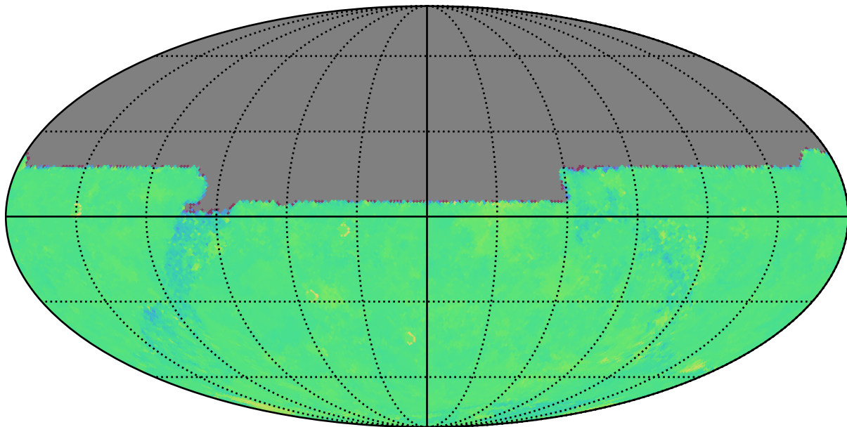
ddf_loaded_half_fl15_v3.3_10yrs u: Kuiper rotTelPos
