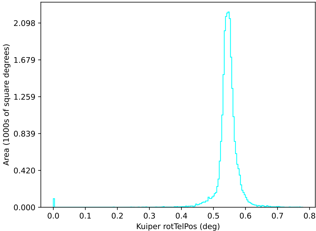
ddf_loaded_half_fl15_v3.3_10yrs u: Kuiper rotTelPos
