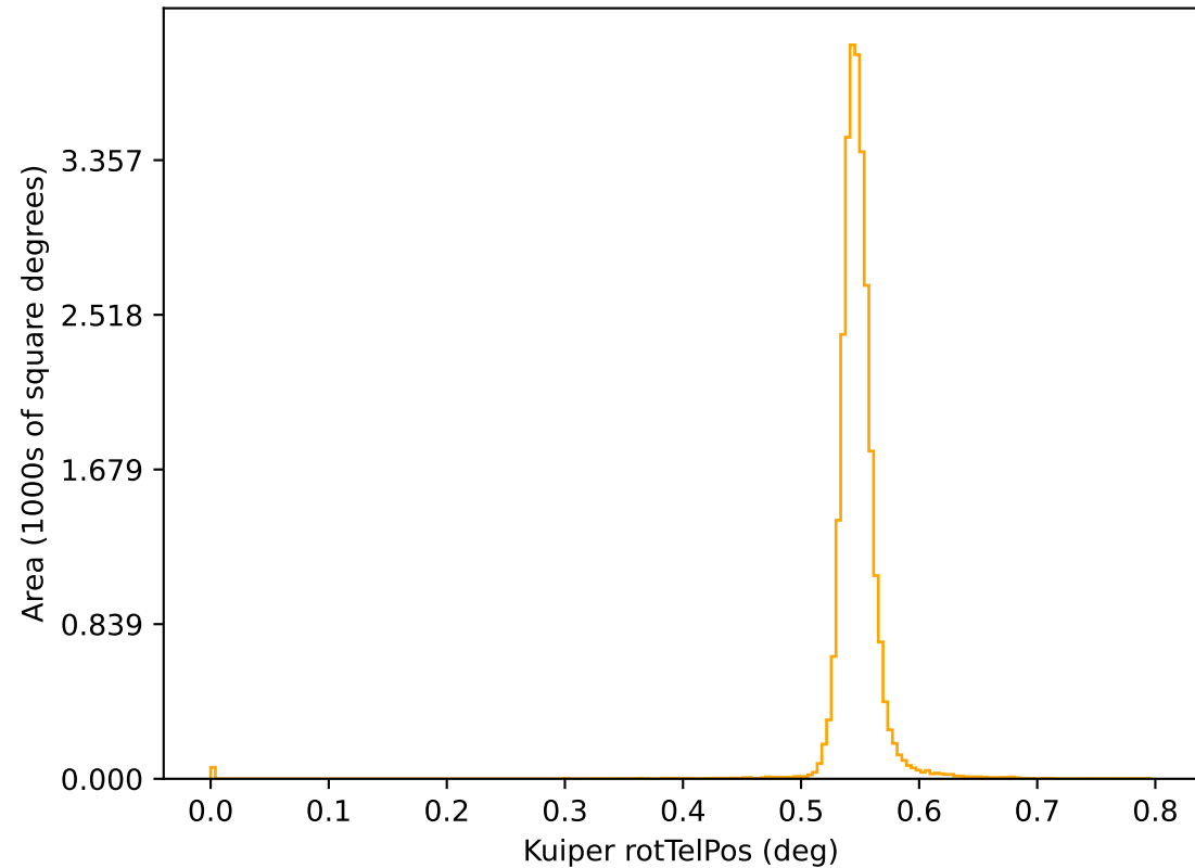
ddf_loaded_half_fl15_v3.3_10yrs r: Kuiper rotTelPos
