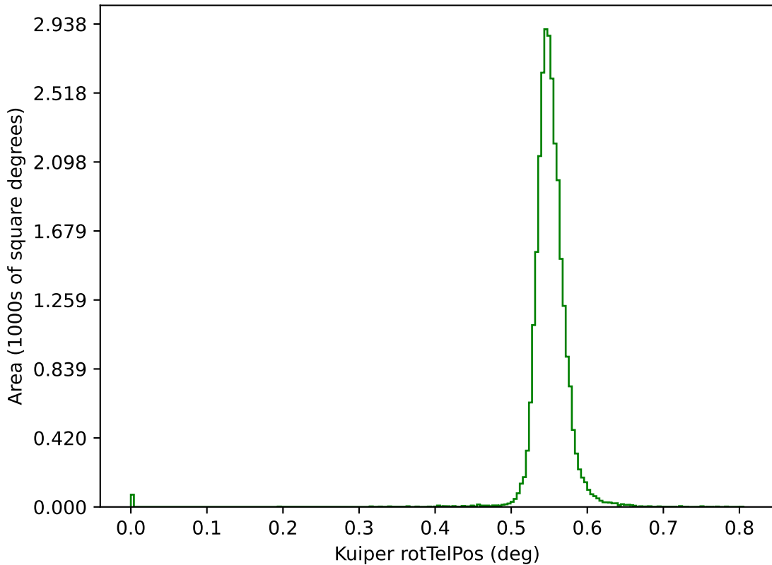
ddf_loaded_half_fl15_v3.3_10yrs g: Kuiper rotTelPos
